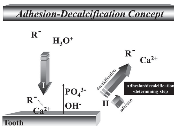
Fig. 17 Schematic illustration of the Adhesion-Decalcification concept or 'AD-concept'. After ionic interaction of the functional monomer (usually a carboxyl or phosphate group), there are two options: either the ionic bond is hydrolytically stable, resulting in a Ca-monomer salt that can co-polymerize with the monomers of the adhesive resin, or the ionic bond is not stable, resulting in decalcification and release of calcium and phosphate from the tooth surface 55 .
